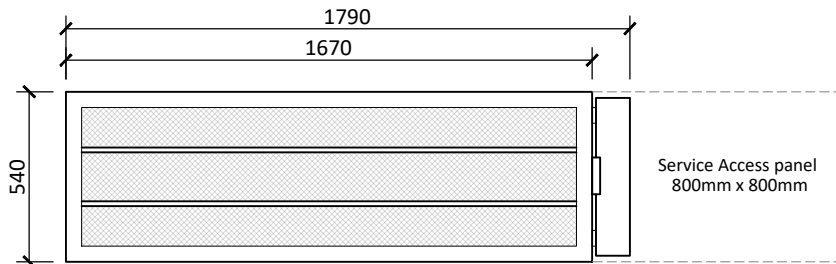
END VIEW
