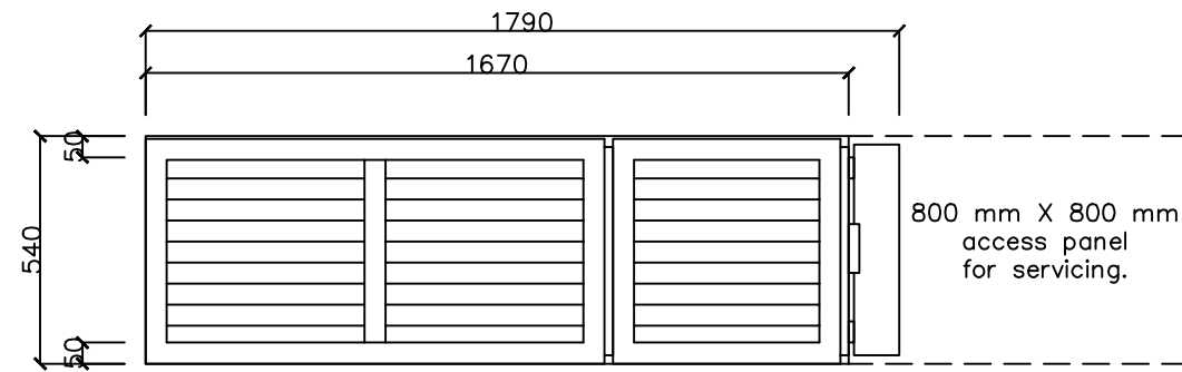
4 END VIEW (OUTLET) Scale 1:20@A3
