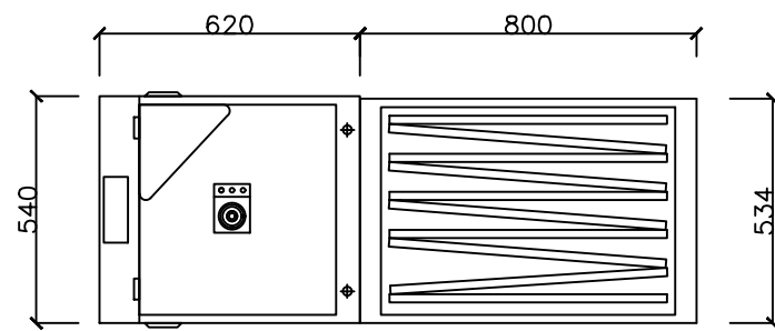
2 FRONT VIEW Scale 1:20@A3
