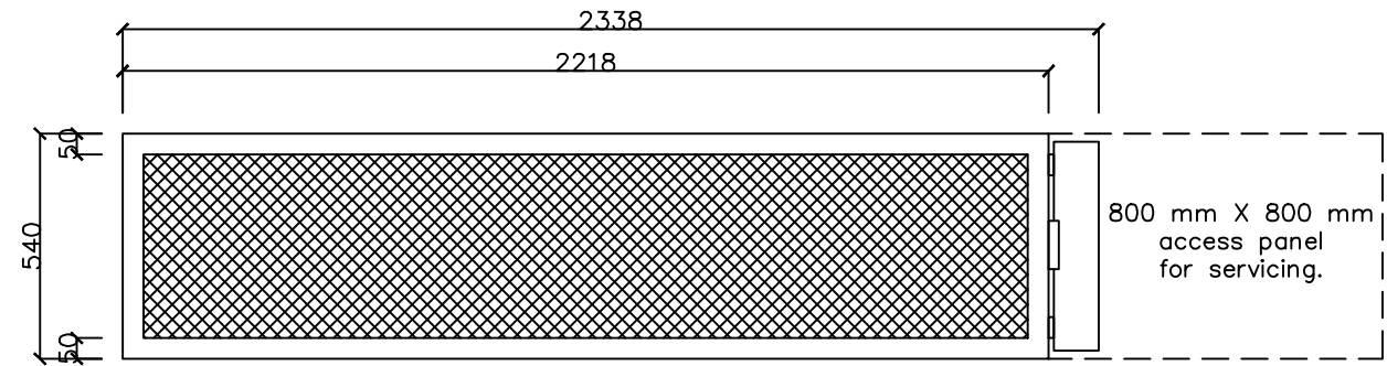
3 END VIEW (INLET) Scale 1:20@A3
