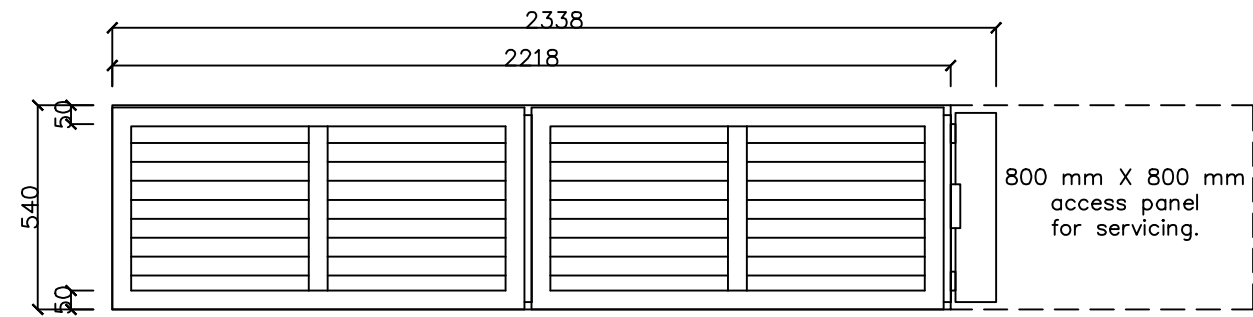
4 END VIEW (OUTLET) Scale 1:20@A3
