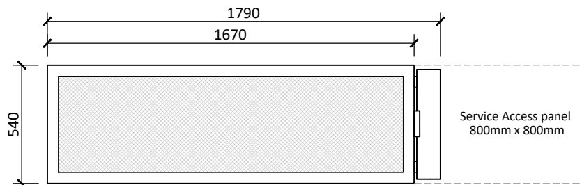
END VIEW
